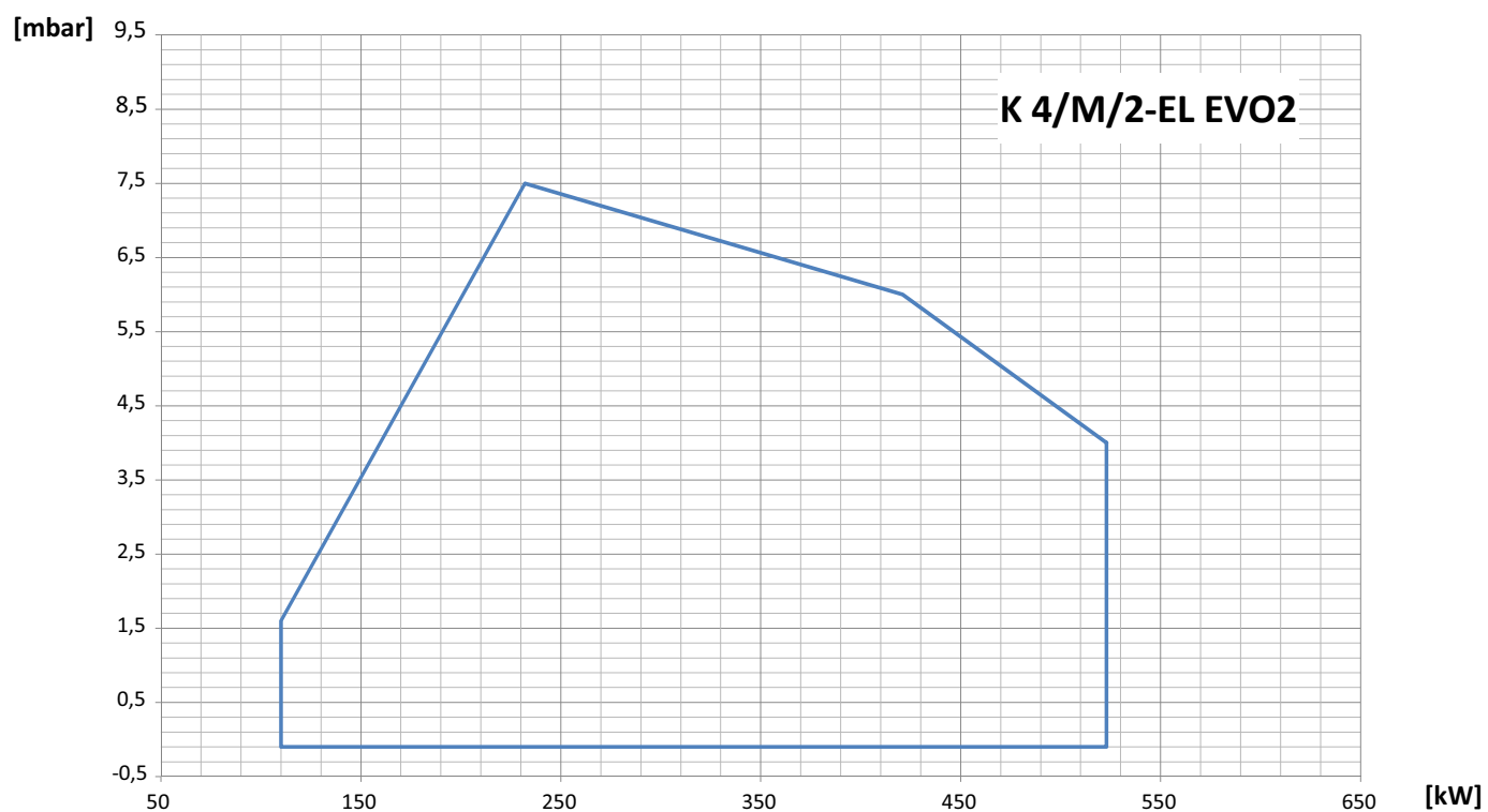
Fig. X = Thermal power Y = Pressure in combustion chamber
