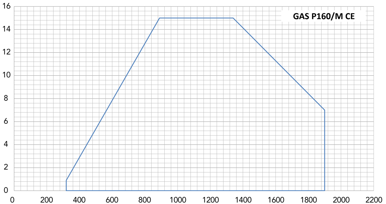
Fig. X = Thermal power [kW] Y = Pression in the combustion chamber [mbar]
