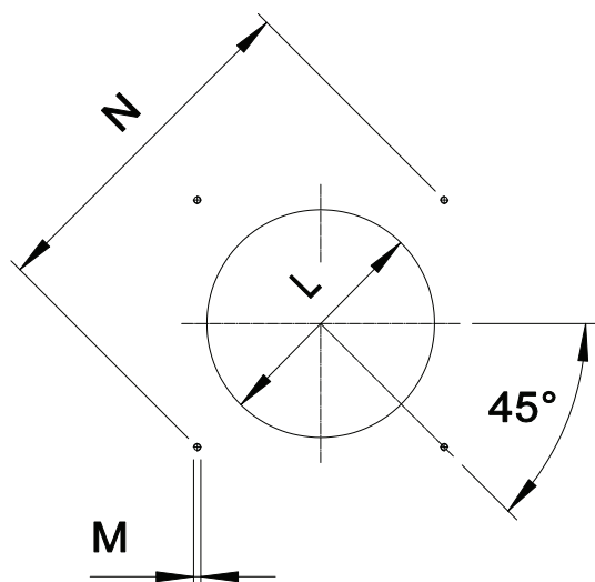
Fig. 6 Boiler plate
