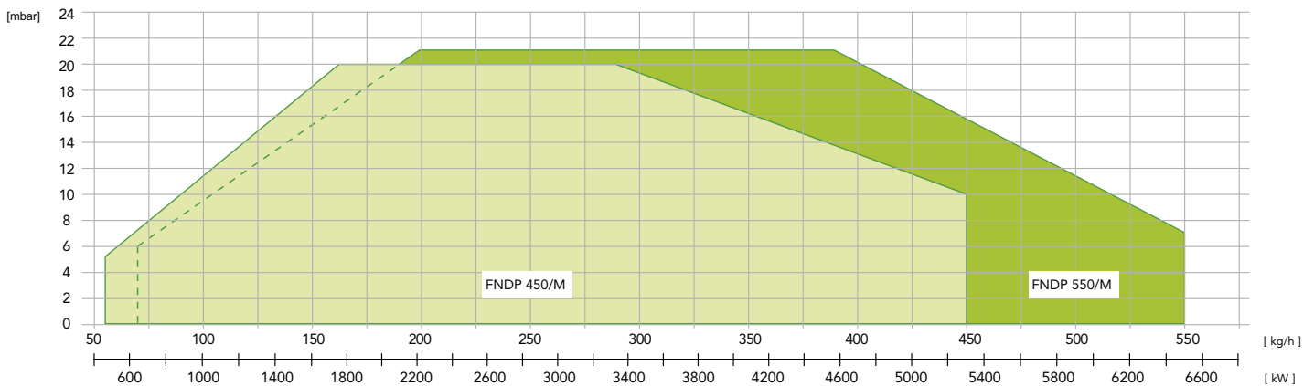
Fig. 5 X = Flow/Thermal power Y = Pression in the combustion chamber
