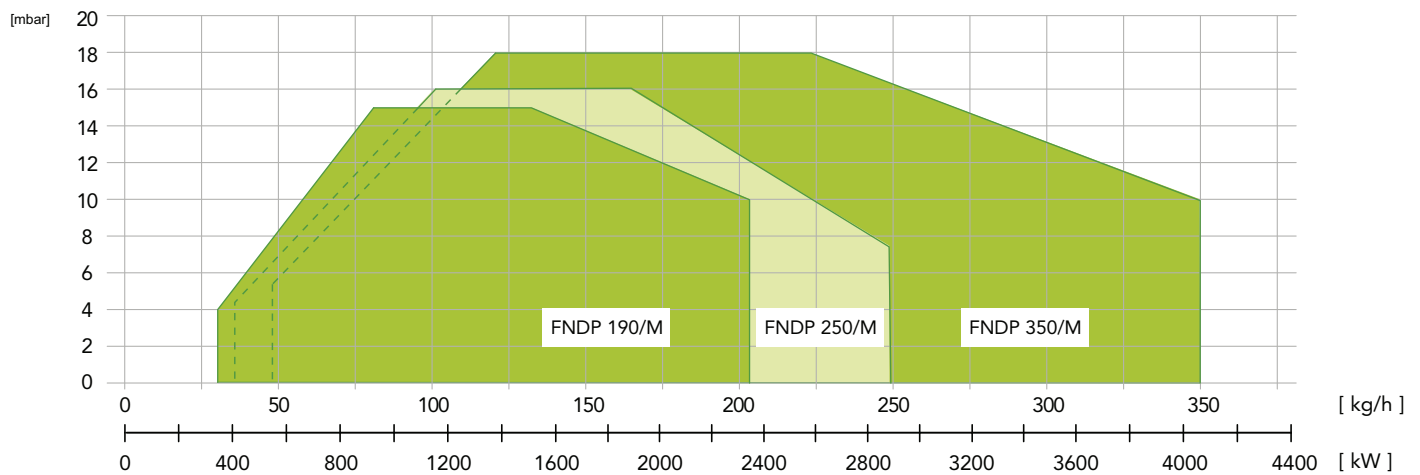
Fig. 4 X = Flow/Thermal power Y = Pression in the combustion chamber
