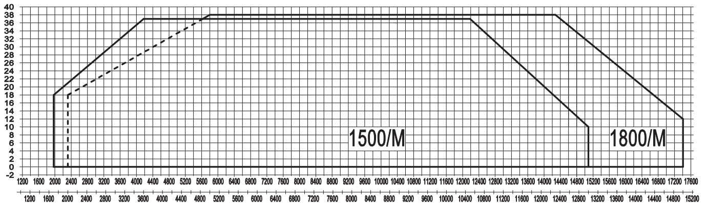
Fig. 3 X = Thermal power (kW - Mcal/h) Y = Pressure in the combustion chamber (mbar)
