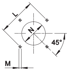
Fig. 4 Boiler plate
