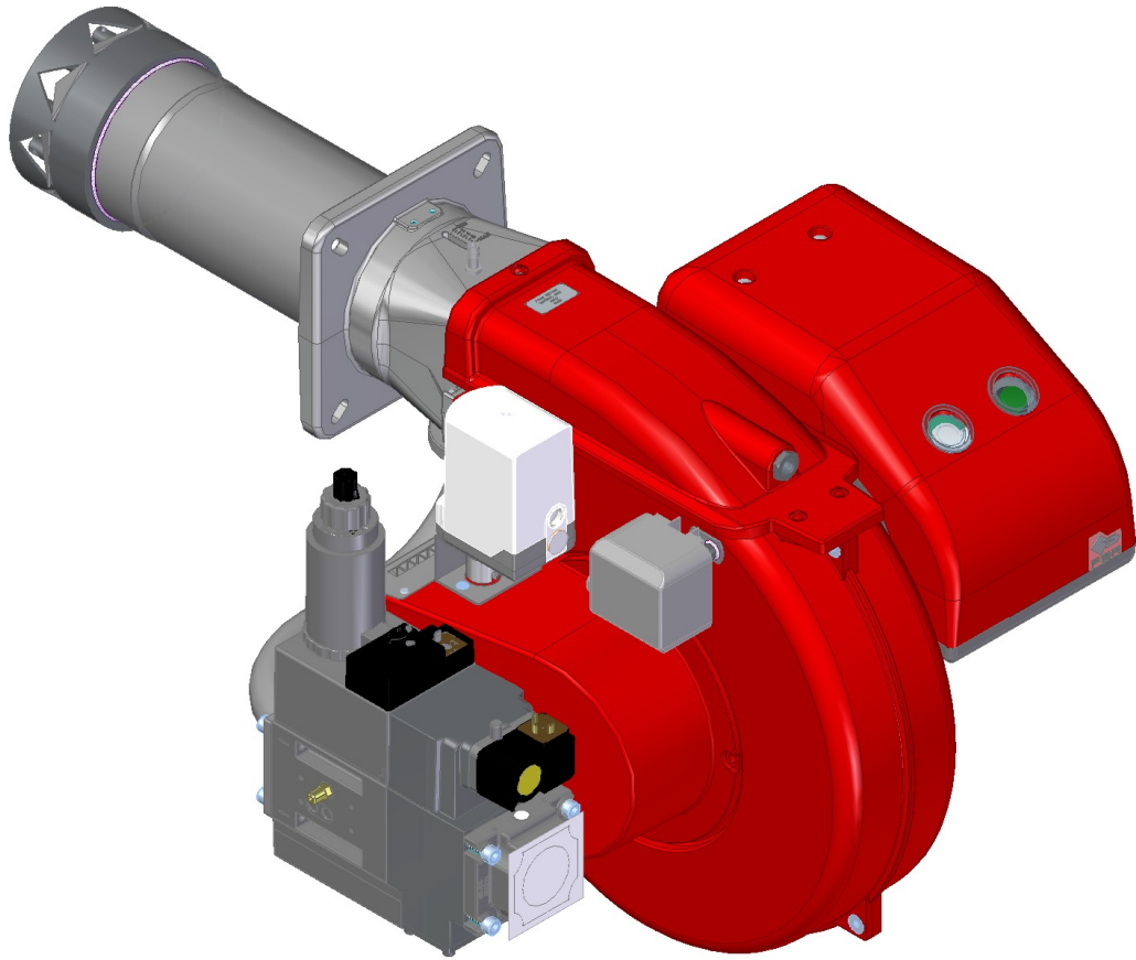
Fig. 1 GAS XP60/2CE-LX-EVO
