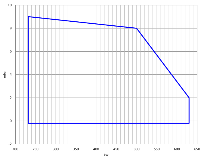
Fig. 2 X = Thermal power Y = Pression in the combustion chamber
