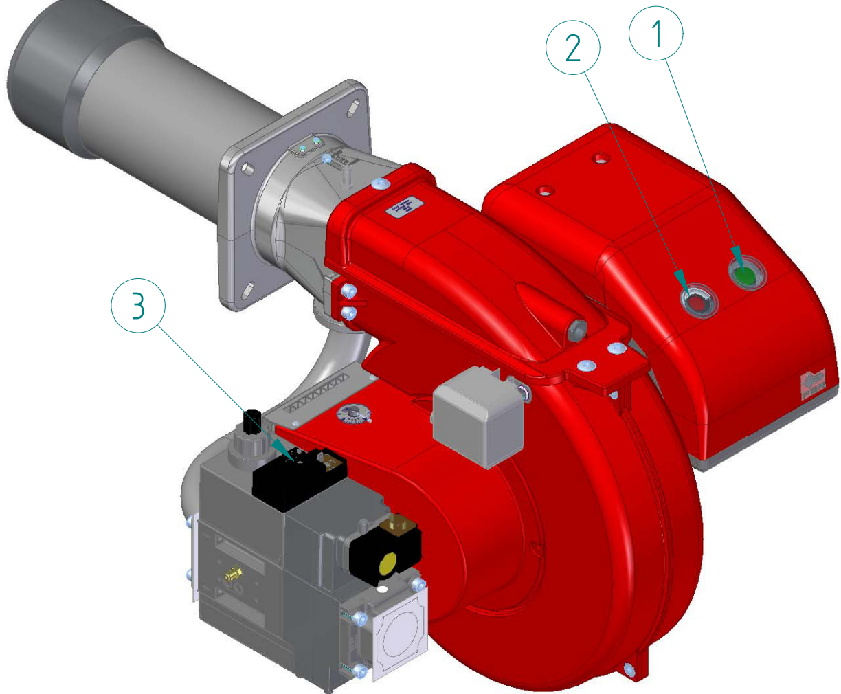
Fig. 5 Burner signal description
