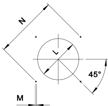
Fig. 4 Boiler plate
