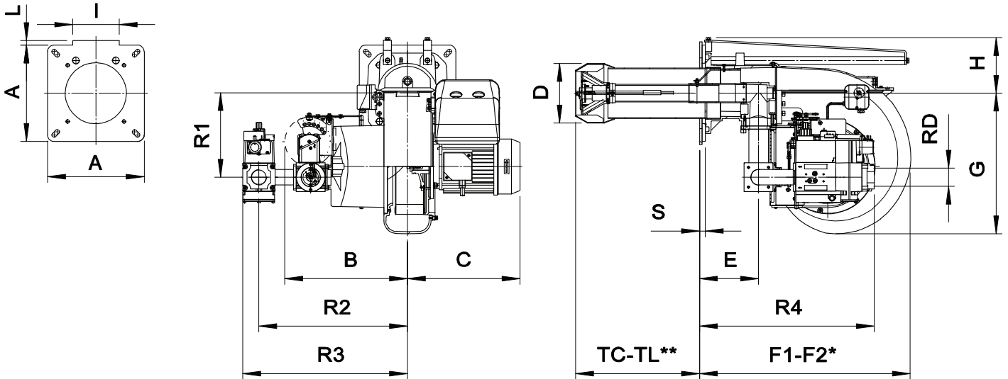
Fig. 5 GAS P100/MCE-LX
