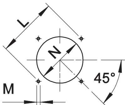
Fig. 7 Boiler plate
